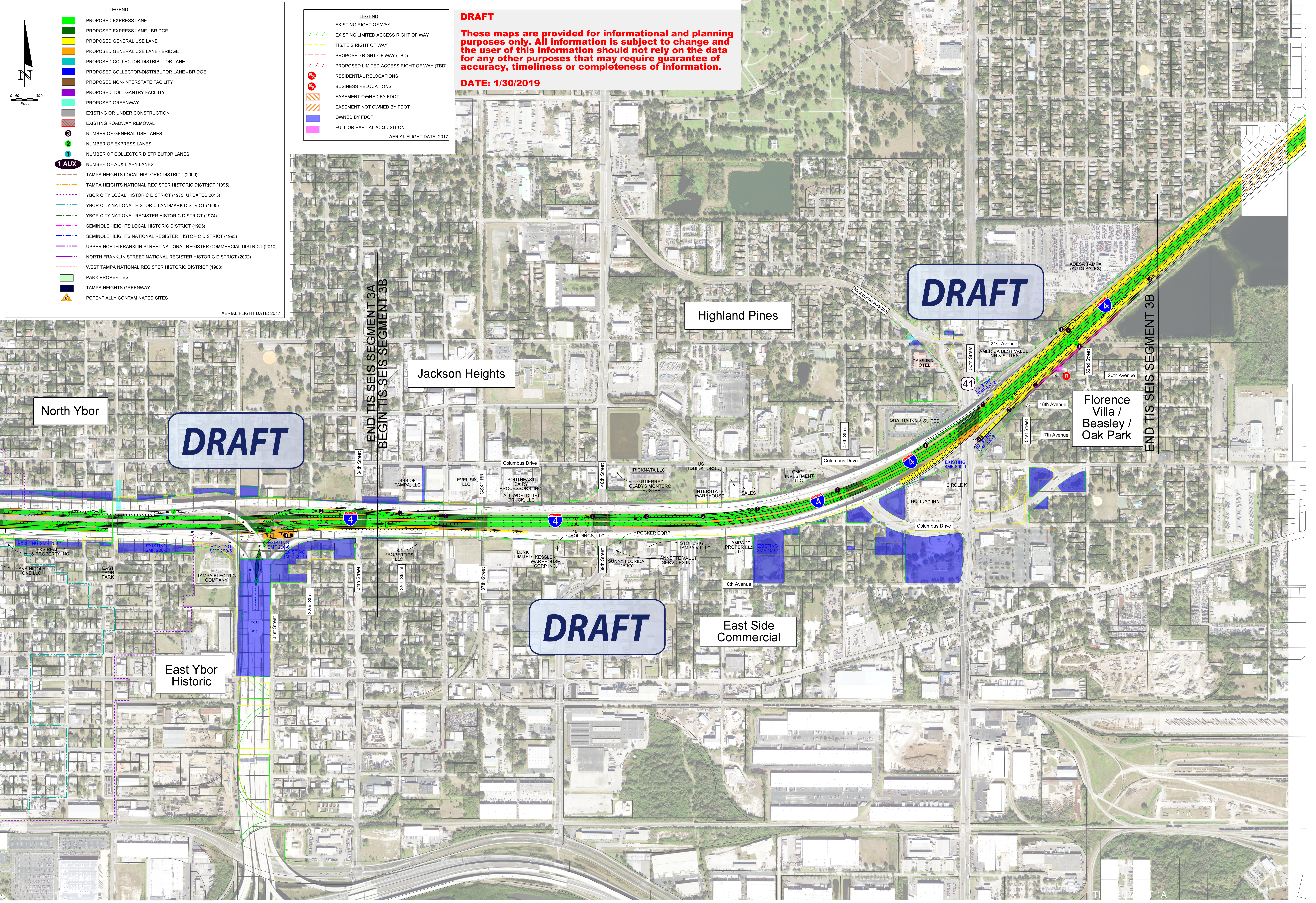
TIS SEIS SEGMENT 3B - CONCEPTUAL ALTERNATIVE ALIGNMENT
